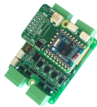
IoTextra Octal3 with IoTsmart ESP32-S3
